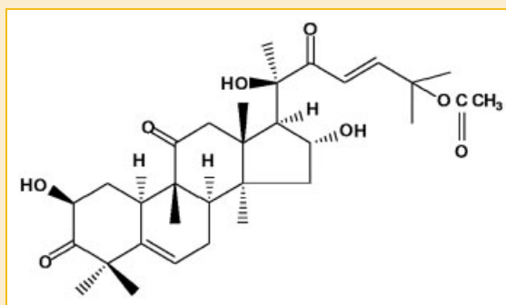
Fig. 1. Chemical structure of cucurbitacin B isolated from the Trichosanthes kirilowii .
